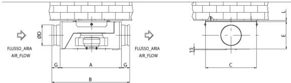
MODELLI / MODELS 100 / 125 / 150
