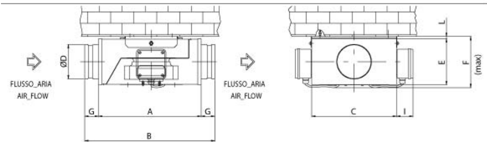
MODELLI / MODELS 200 / 250 / 315
